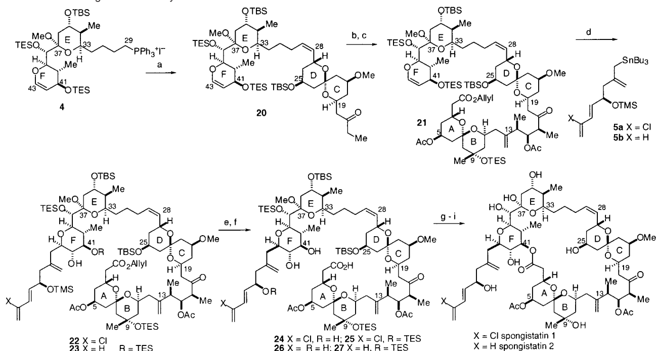
Scheme 3: Final Fragment Assembly a
